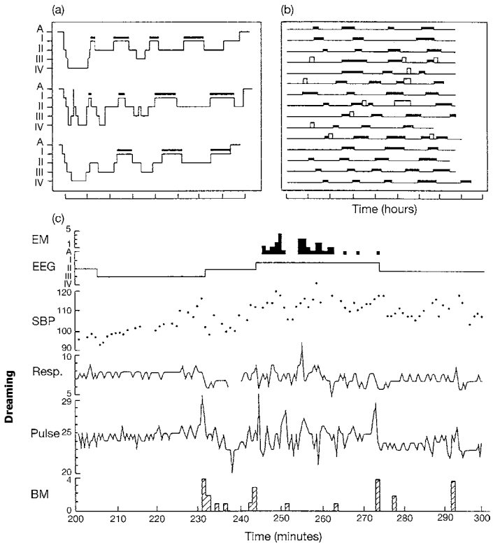
7. Sleep cycle with activation. (A, B) Ultradian sleep cycle of NREM and REM sleep shown in detailed sleep-stage graphs of 3 human subjects (A) and REM sleep periodograms of 15 human subjects (B). In (C) one such sleep cycle is shown to illustrate the changes in eye movements (EM), EEG, blood pressure (SBP), respiration (resp.), pulse, and body movements (BM) that are associated with REM.
