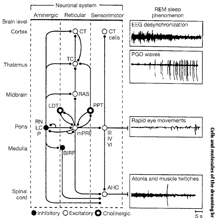
4. Schematic representation of the REM sleep generation process. A distributed network involves cells at many brain levels (left). The network is represented as comprising three neuronal systems (centre) that mediate REM sleep electrographic phenomena (right).
